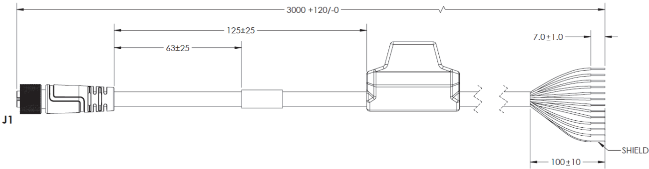
SCHEMATIC
