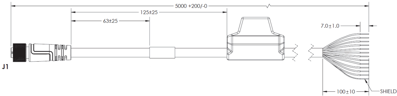
SCHEMATIC
