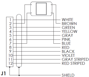
SCHEMATIC
