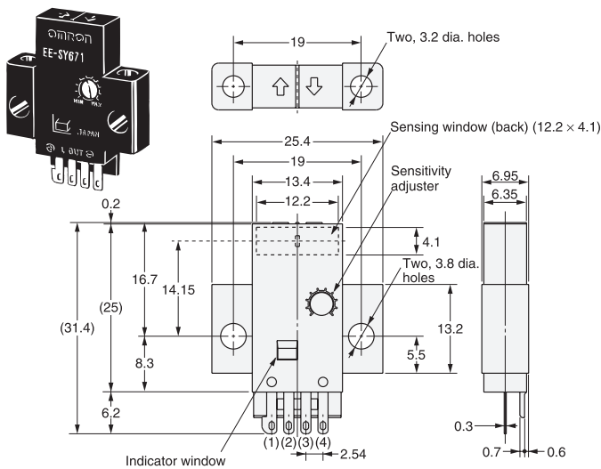
Terminal Arrangement
