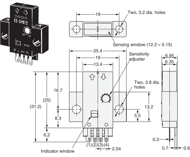
Terminal Arrangement
