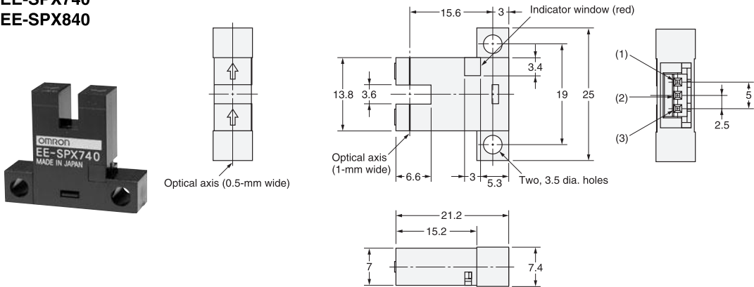
Terminal Arrangement
