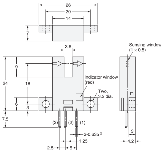
Terminal Arrangement
