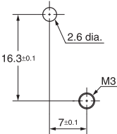
Mounting screw holes
