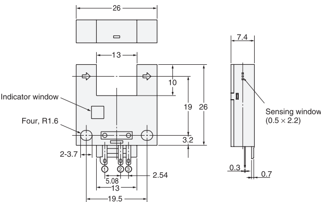
Terminal Arrangement
